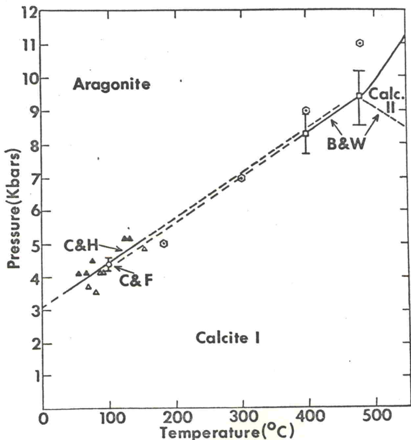
FIG. 1. Calcite-Aragonite Equilibrium Curves. Solid triangle, run product = aragonite; open triangle, run product = calcite; line labeled C and H, equilibrium curve established by this paper. Open circle labeled C and F, equilibrium point established by Crawford and Fyfe (1964). Open squares, equilibrium points established by Boettcher and Wyllie (1968). Line labeled B and W, equilibrium curves established by Boettcher and Wyllie. Bars extending from open symbols denote limits of experimental error. Open hexagons, equilibrium points established by Johannes and Puhan (1971). Size of hexagon indicates approximate limit of experimental error. Curve extrapolations dashed.
